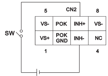
External Power Source I=6~20mA
